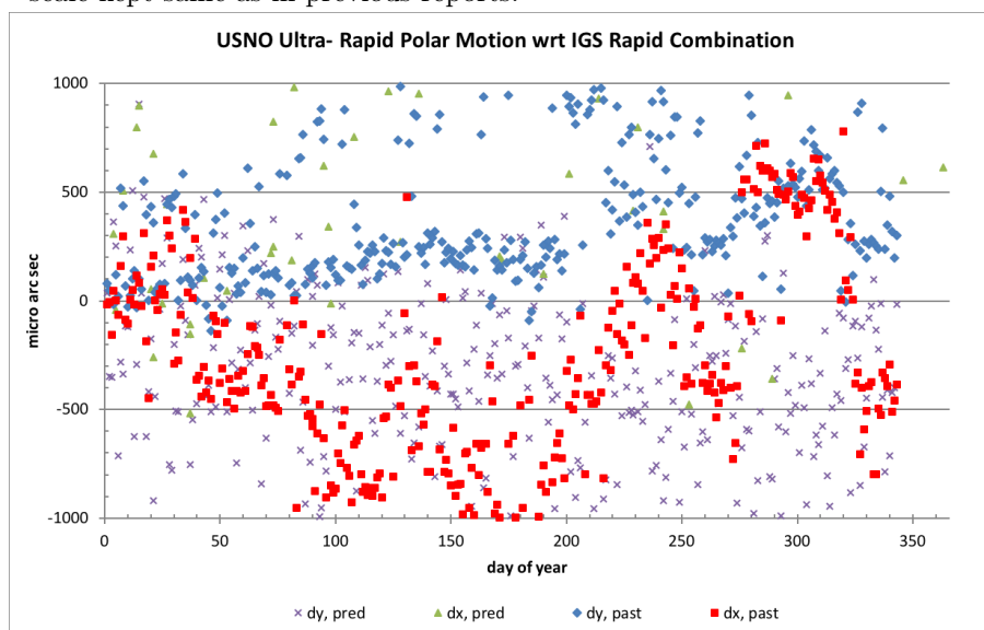
Figure 4: USNO Ultra-rapid polar motion estimates minus IGS Rapid Combination values, 2019.
