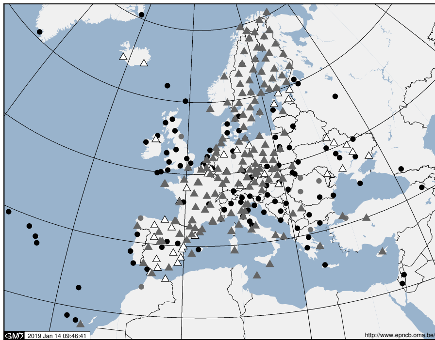
Figure 3: EPN tracking stations (status Dec. 2018). : ● tracking only GPS, ●: tracking GPS+GLONASS, Δ: tracking GPS+GLONASS+Galileo, and ▲: tracking GPS+GLONASS+Galileo+BeiDou.
