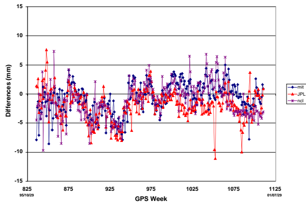
Penticton (DRAO) Height differences (IGS-GNAAC) Figure 7
