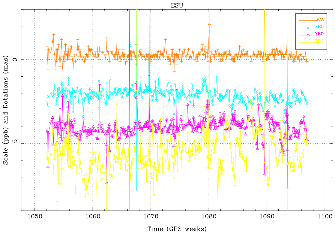
Figures 23a,b: Daily Transformation parameters of the ESA Ultra Rapid orbits w.r.t. the IGS Rapid orbits. Translations are shifted by 50 mm, Rotations are shifted by 2 mas.
