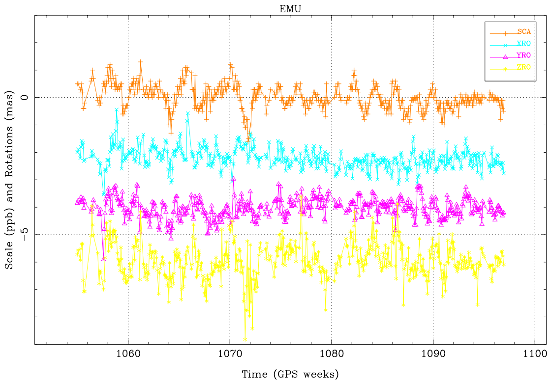
Figures 22a,b: Daily Transformation parameters of the EMR Ultra Rapid orbits w.r.t. the IGS Rapid orbits. Translations are shifted by 50 mm, Rotations are shifted by 2 mas.
