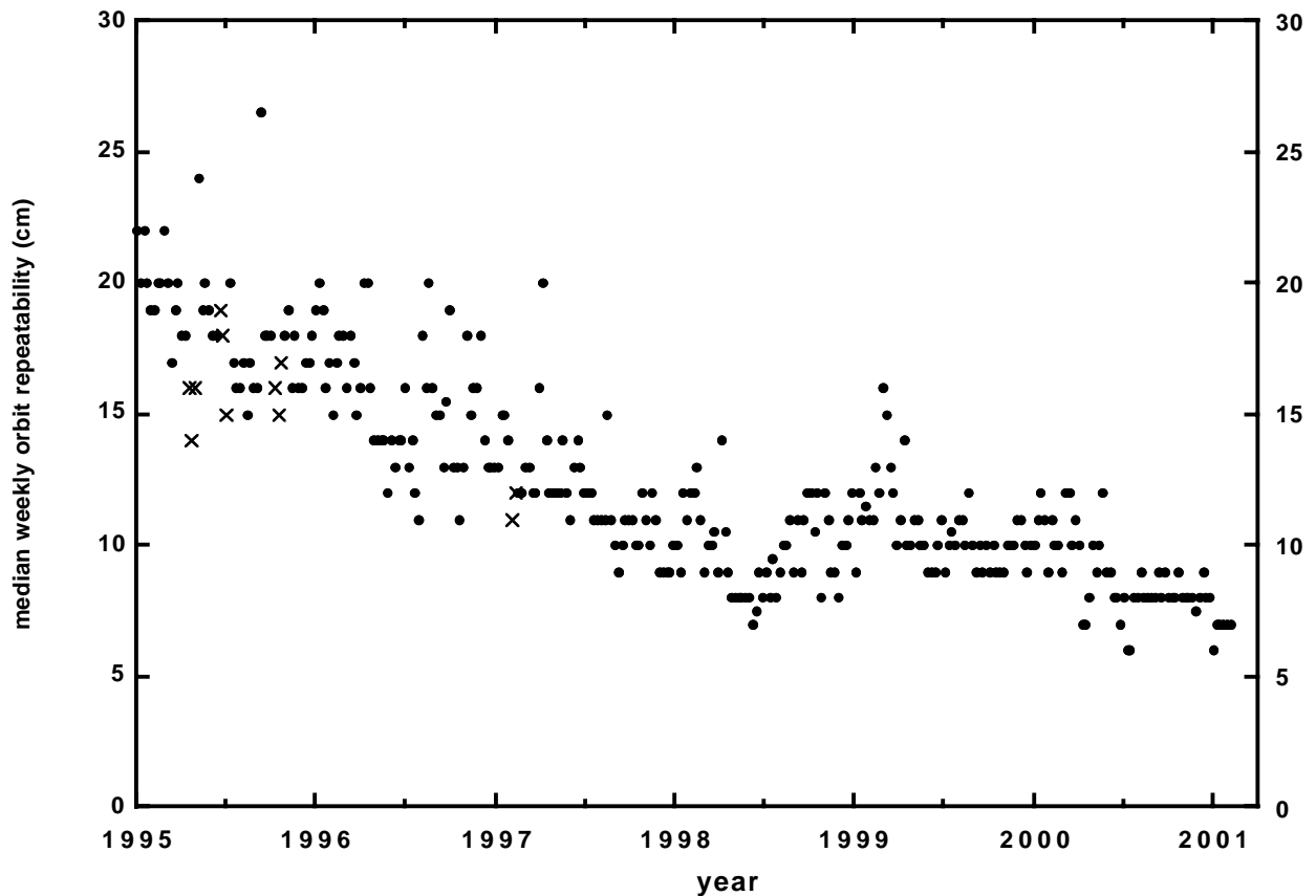
Figure 1: JPL orbit repeatability (3drms) since 1995. Each data point represents the median over all satellites and days for a particular GPS week. (The daily number for a given satellite indicates the degree to which the precise orbit agrees with those of adjacent days near the midnight boundary.) Weeks during which AS was off are indicated with an 'X'.
