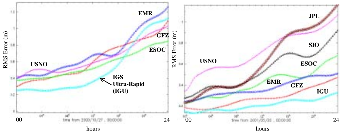
Figure 6: Epoch by epoch unweighted RMS error of predicted part of Ultra-Rapid AC submissions and the IGU versus the IGR for October 26 th ,2000 (00300) on the left and May 19 th , 2001 (01139) on the right.
