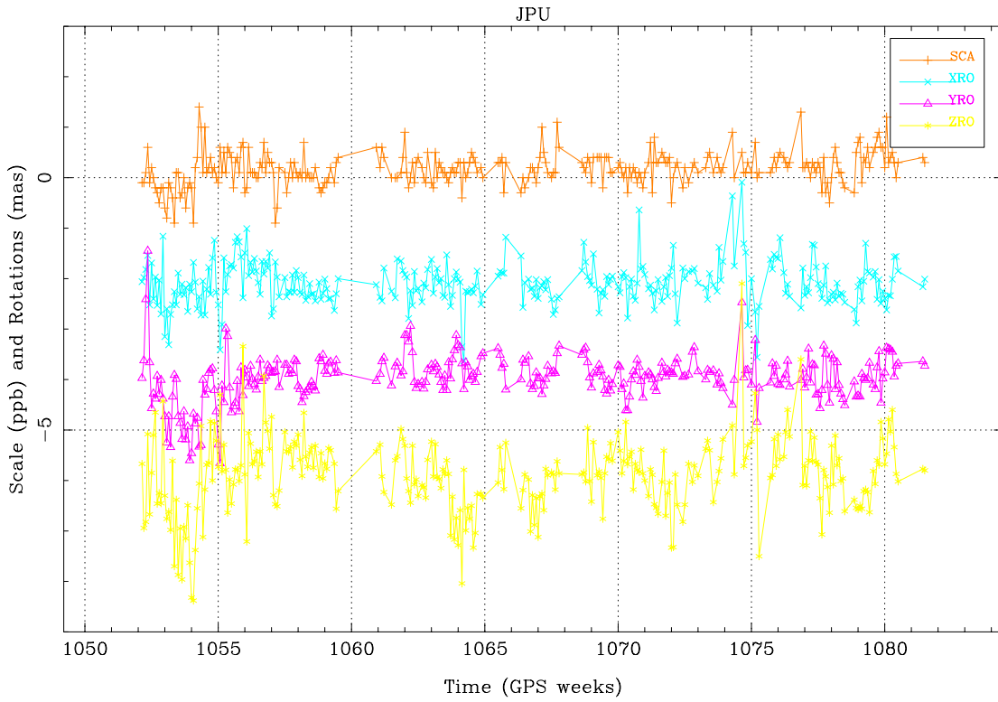
Figures 25a,b: Daily Transformation parameters of the JPL Ultra Rapid orbits w.r.t. the IGS Rapid orbits. Translations are shifted by 50 mm, Rotations are shifted by 2 mas.
