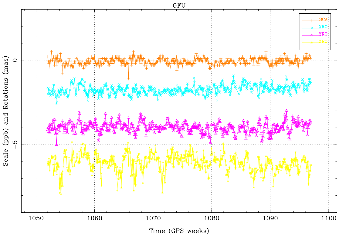
Figures 24a,b: Daily Transformation parameters of the GFZ Ultra Rapid orbits w.r.t. the IGS Rapid orbits. Translations are shifted by 50 mm, Rotations are shifted by 2 mas.
