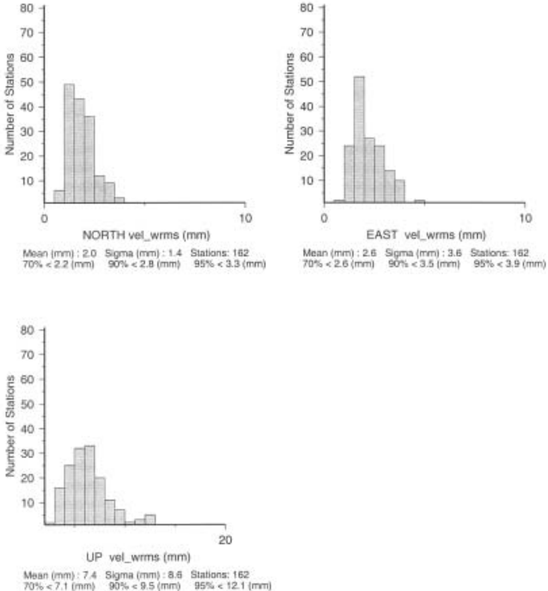
Figure 2. Histograms of the RMS scatter of the site position estimates (about a linear regression) from the weekly IGS combined SINEX files. In North, East and Up the median RMS scatters are 1.8, 2.0, and 6.2 mm, respectively.
