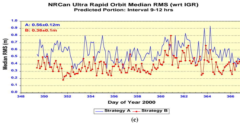
Figure 2: NRCan Ultra Rapid Orbit Median RMS (wrt IGR) for Strategies A and B during December 14-31, 2000.
