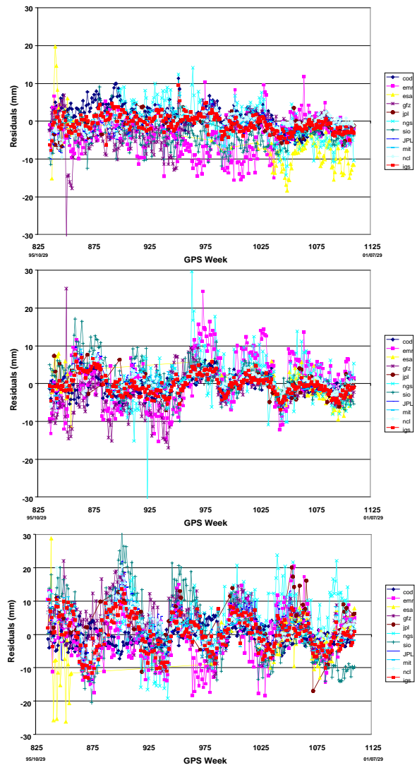
Figures 6 a-b-c. Latitude, Longitude and Height residuals between the weekly and cumulative solutions at station Penticton (DRAO)
