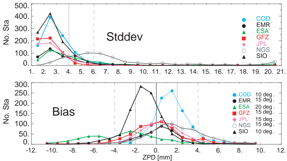
Figure 5. Differences in the zenith path delay between the individual GPS estimates and the IGS Combined Product. Histograms of standard deviation and bias for the GPS weeks 1080 to 1087.
