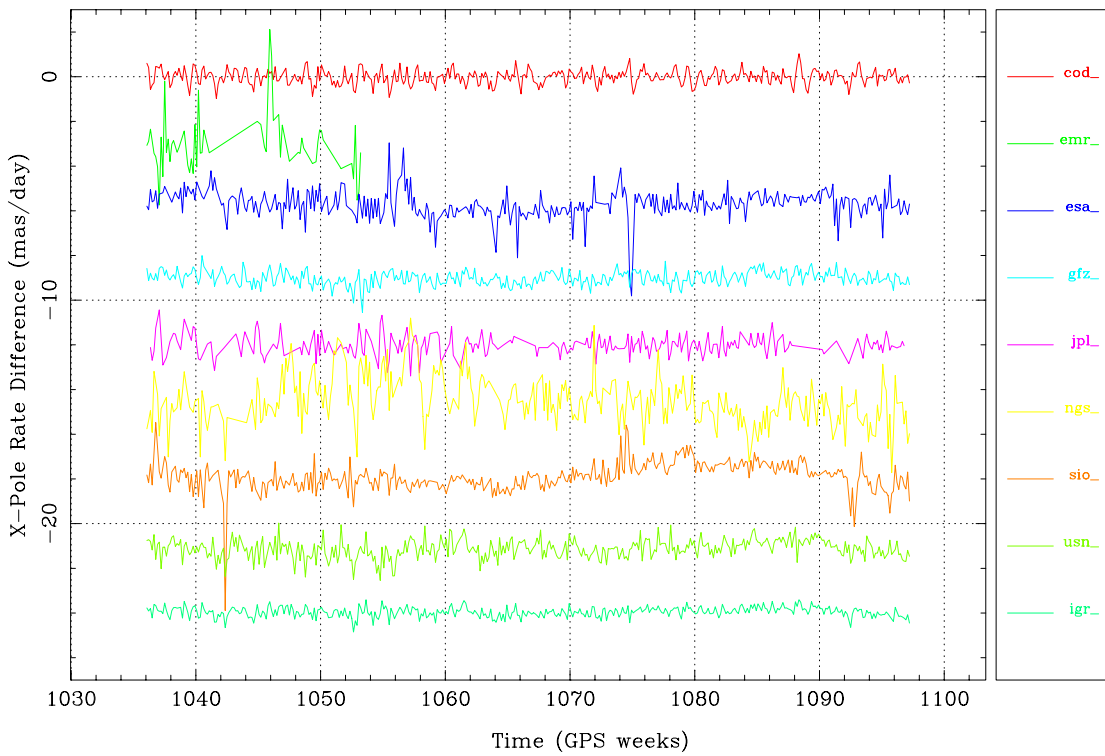
Figure 36: Daily AC Rapid x-Pole-rate Differences w.r.t. the IGS Final x-Pole-rates. ACs are shifted by 3 mas/day.
