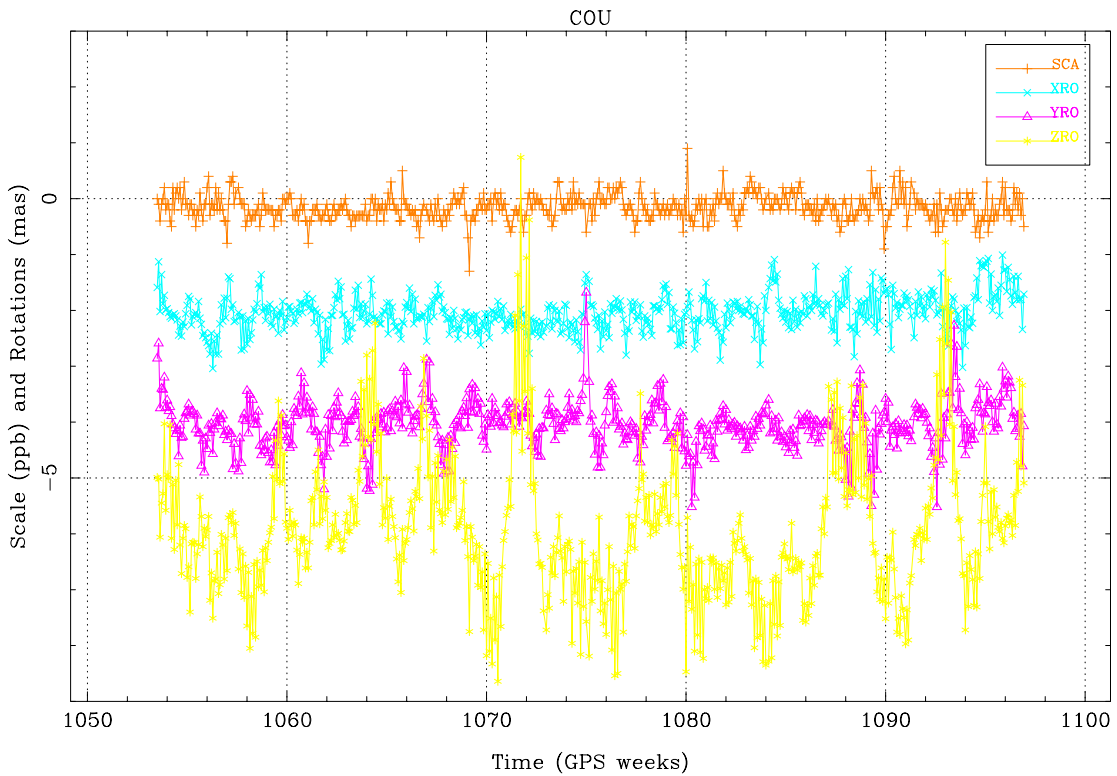
Figures 21a,b: Daily Transformation parameters of the COD Ultra Rapid orbits w.r.t. the IGS Rapid orbits. Translations are shifted by 50 mm, Rotations are shifted by 2 mas.
