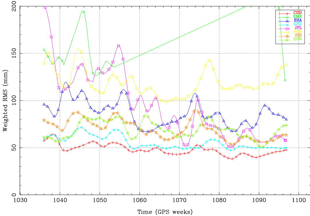
Figure 3: Weighted orbit RMS(mm) of the Rapid AC submission w.r.t the IGS Rapid combination. The daily RMS values of the combination summaries were smoothed for plotting purposes, using a sliding 7 day window.
