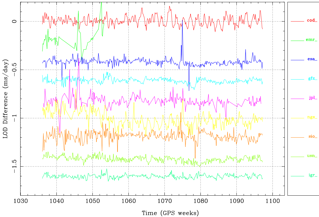
Figure 38: Daily AC Rapid LOD Differences w.r.t. the IGS Final Pole. ACs are shifted by 0.2 ms/day.
