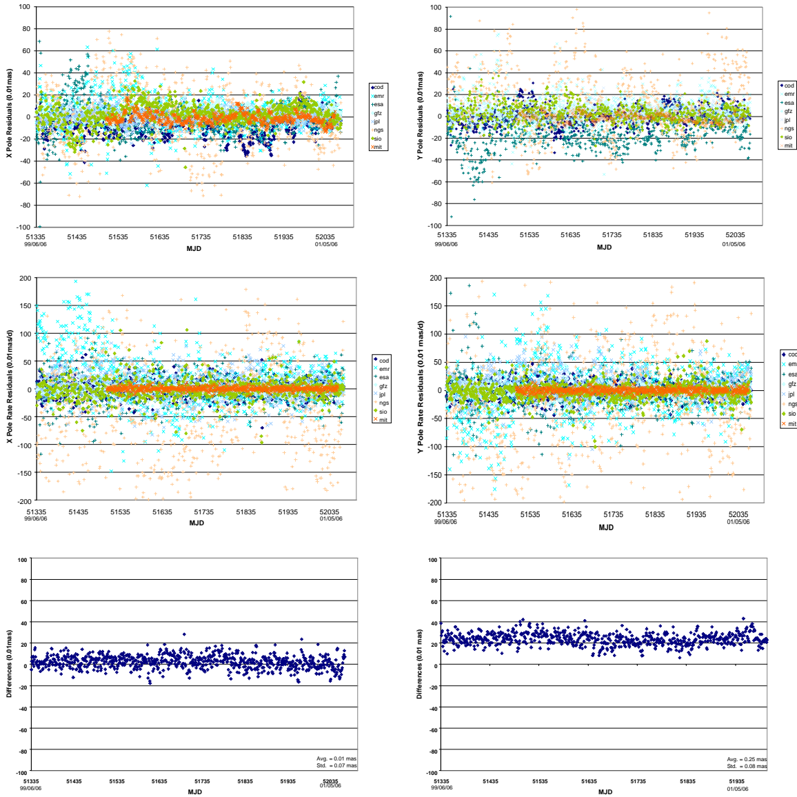
Figure 11 a-b (top) c-d (middle) e-f (bottom). Daily X Pole, Y Pole, (top) X Pole Rate, Y Pole Rate (middle) differences between the combined solution “igs00P02” and the AC/GNAAC estimates. Daily X Pole, Y Pole, (bottom) differences between the combined solution “igs00P02” and the Bulletin A.
