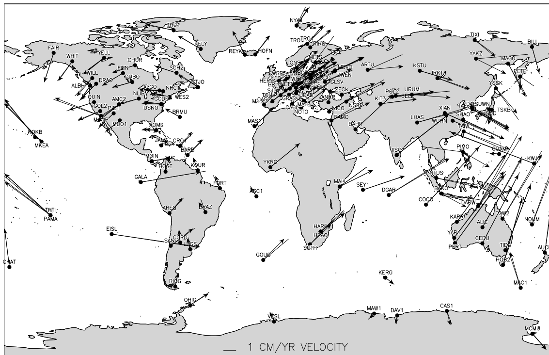
Figure 1: Velocity vectors estimates from a constrained solution (arrows) and from ITRF97 (lines).
