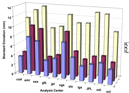
Figure 5. AC/GNAAC Station Coordinates Residuals STD with respect to the Cumulative Solution
