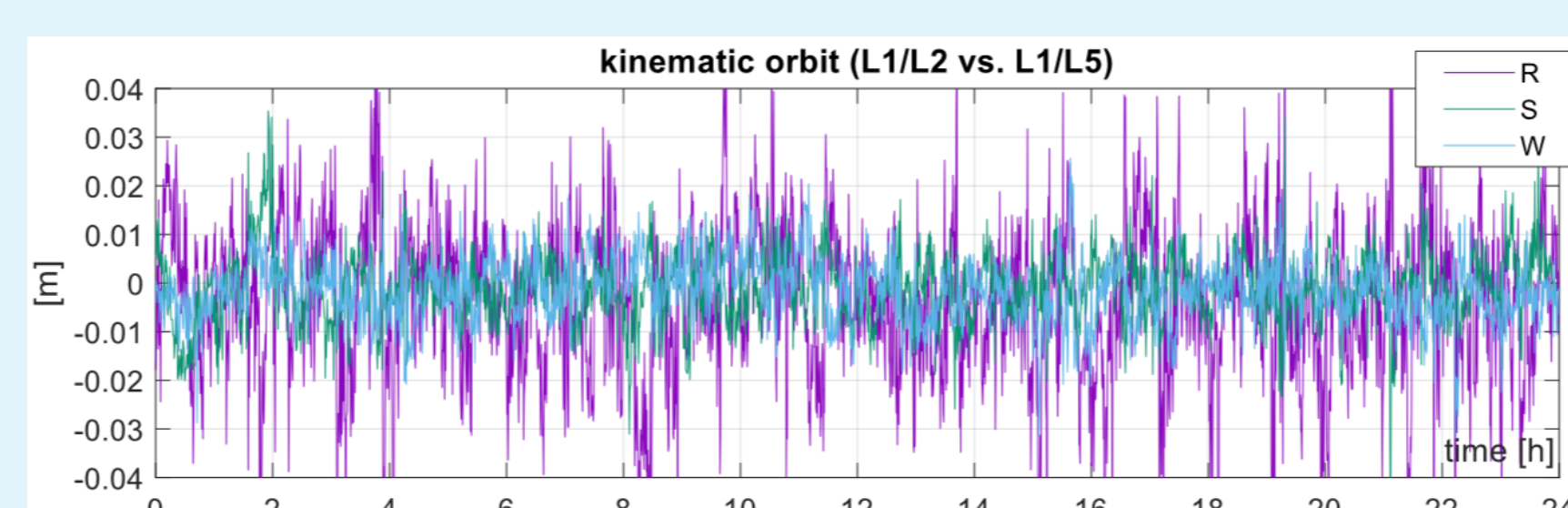
Figure 3: Differences of Sentinel-6A kinematic orbits in radial (R), along-track (S) and cross-track (W) for day 21/062 (when GPS L5 tracking was switched on), once computed with L1/L2 and once with L1/L5.
