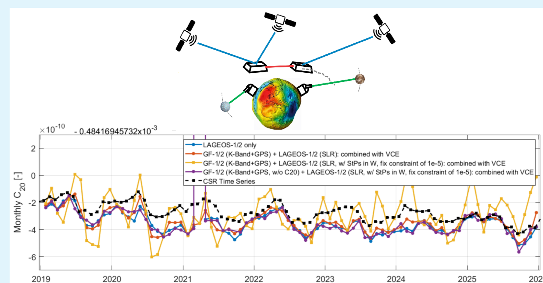
Figure 6: Estimation of the C_{20} coefficient from SLR-only and in combination with GRACE Follow-On data for different combination techniques and pseudo-stochastic orbit parametrisations.
