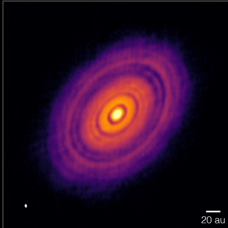
HL Tau
