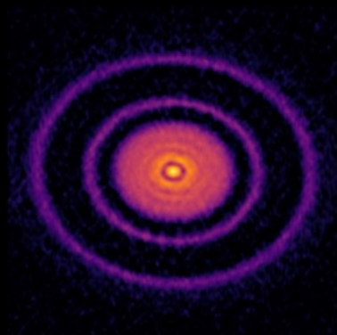
AS 209
