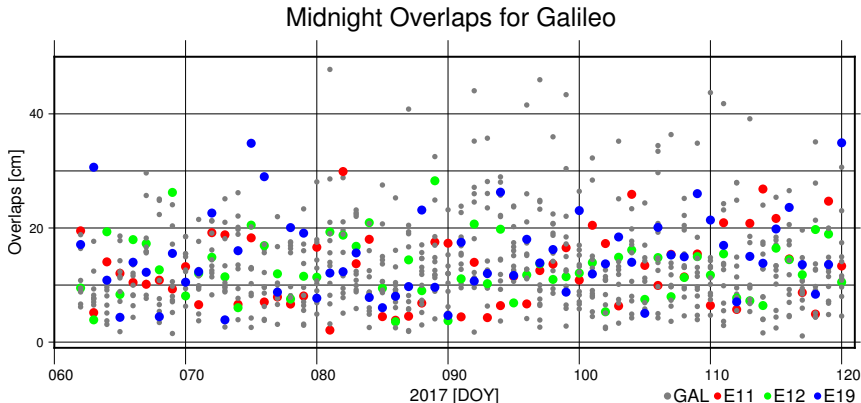
Figure: Midnight overlap of all Galileo satellites (using IGS PCOs)
