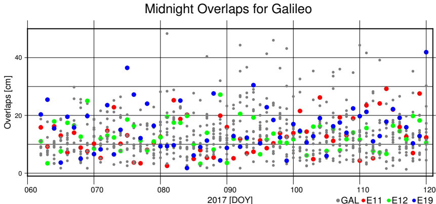
Figure: Midnight overlap of all Galileo satellites (using IOV PCOs and PCVs)
