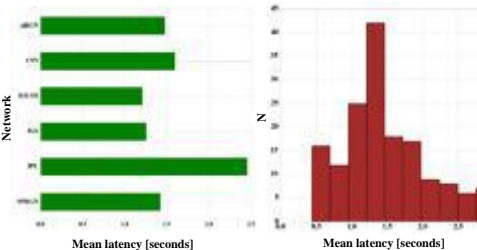
Figure 6: CDDIS data streams grouped by unique network, the mean latency (reported per stream over a single 15 minute observation interval) is averaged over all streams per network and plotted
