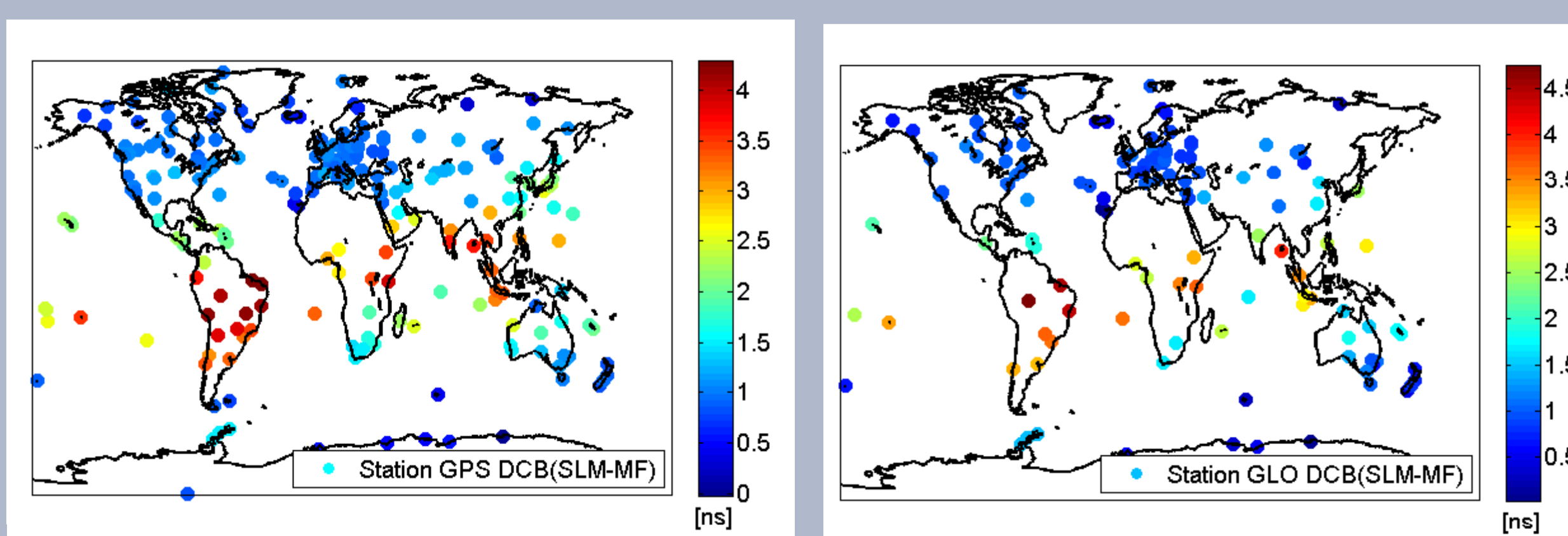
Fig. 3: DCB difference for each stations in ns (left for GPS, right for GLO)
