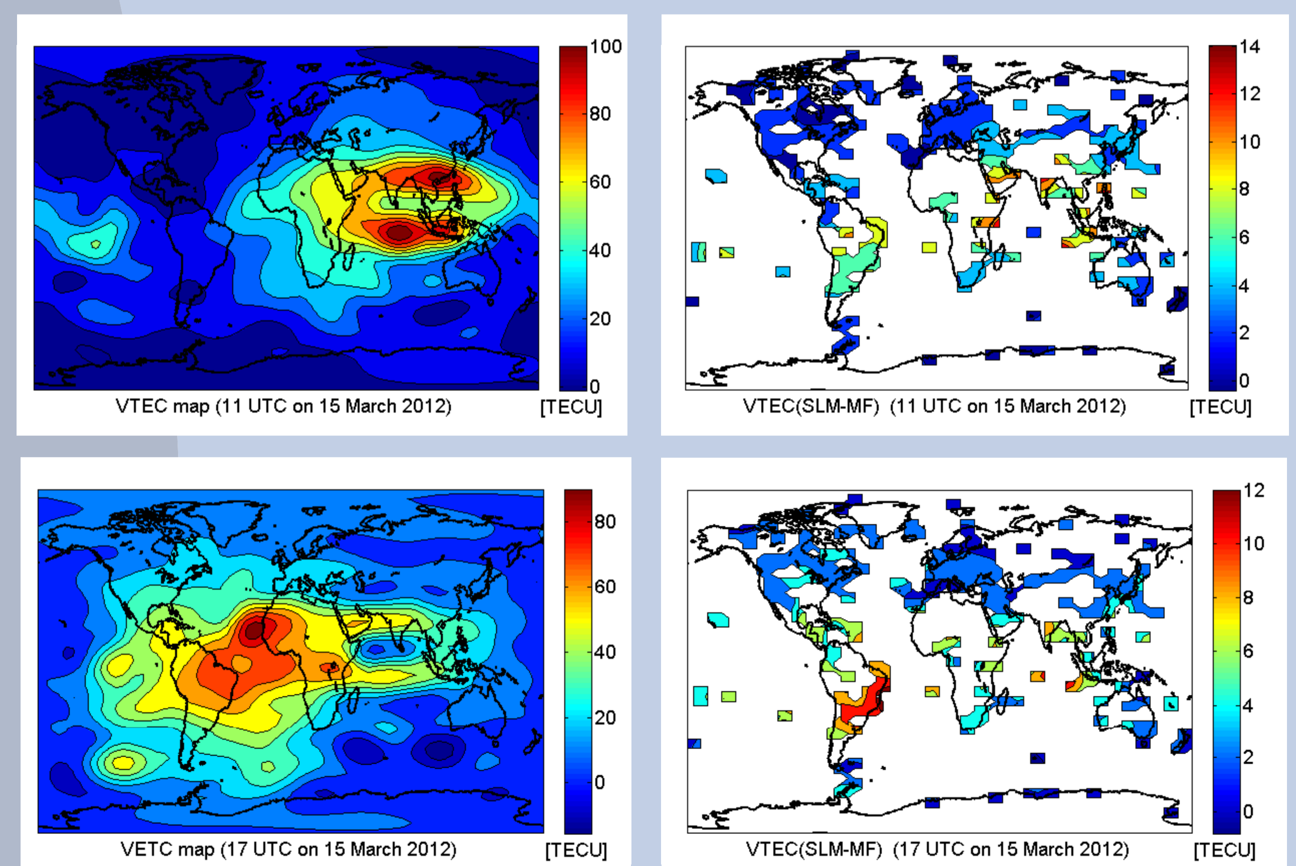
Fig. 4: Left panel: VTEC map [TECU] for two epochs (11 UTC and 17 UTC 15 March 2012). Right panel: VTEC difference [TECU].
