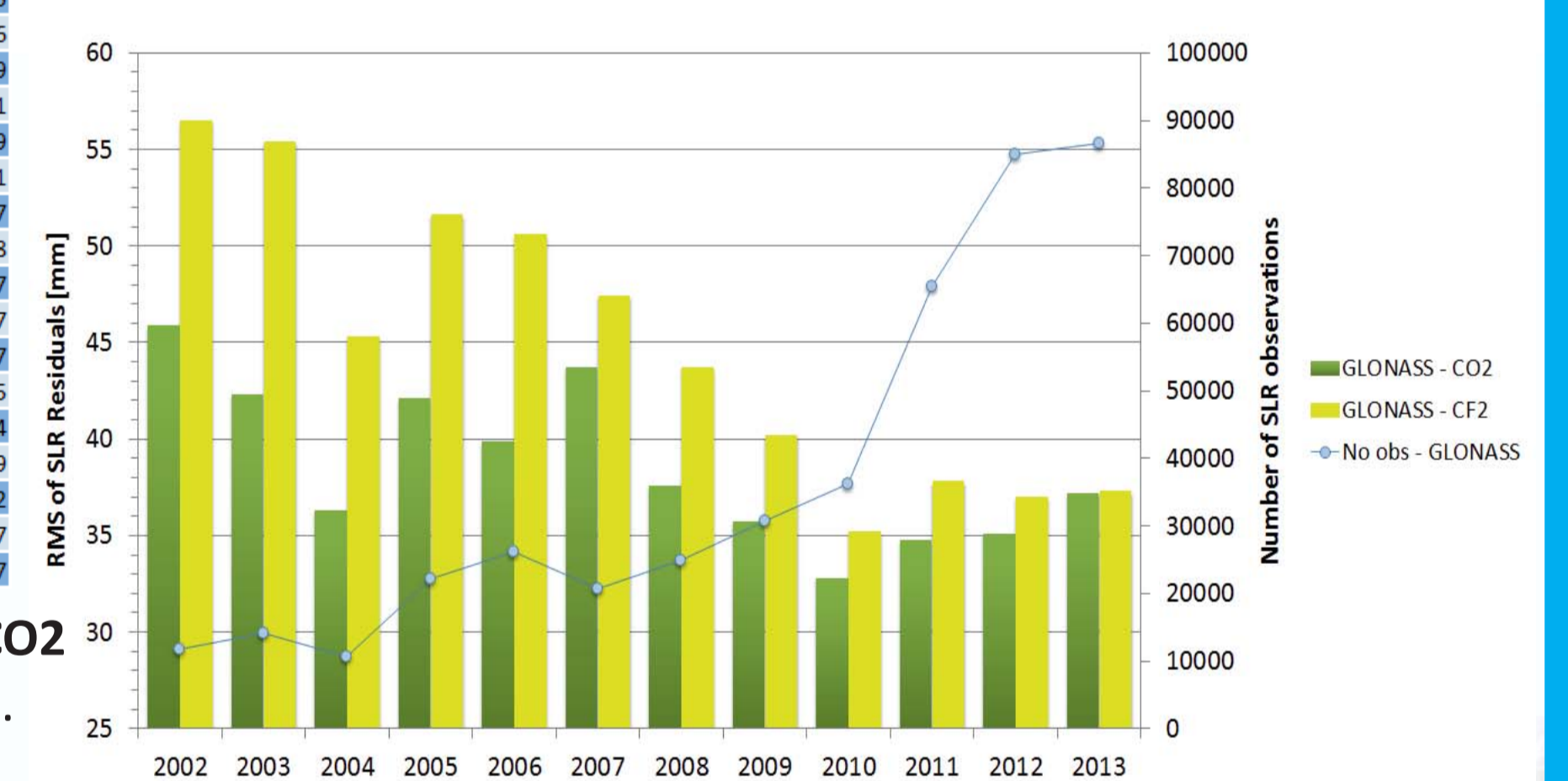
Fig. 6: RMS of SLR residuals to GLONASS satellites for CO2 solutions and CF2 solutions [mm].
