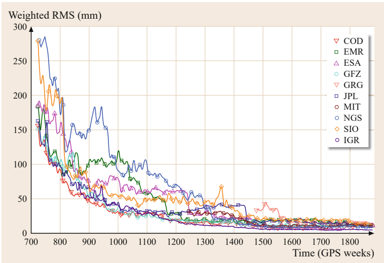
Fig. 33.3 Weighted RMS (mm) of the individual AC orbit solutions with respect to the IGS Final orbits for the period 1994 to Dec. 2015 (smoothed). Individual Analysis Centers are identified by their three-letter acronyms (COD: Center for Orbit Determination in Europe, Switzerland; EMR: Natural Resources Canada; ESA: European Space Agency; GFZ: GeoForschungsZentrum Potsdam, Germany; GRG: Groupe de Recherche de Géodésie Spatiale – Centre National d’Etudes Spatiales (CNES) and Collecte Localisation Satellites (CLS); JPL: Jet Propulsion Laboratory, USA; MIT: Massachusetts Institute of Technology, USA; NGS: National Geodetic Survey, National Oceanic and Atmospheric Administration (NOAA), USA; SIO: Scripps Institute of Oceanography, USA [33.13]). Image courtesy of Geoscience Australia and MIT
