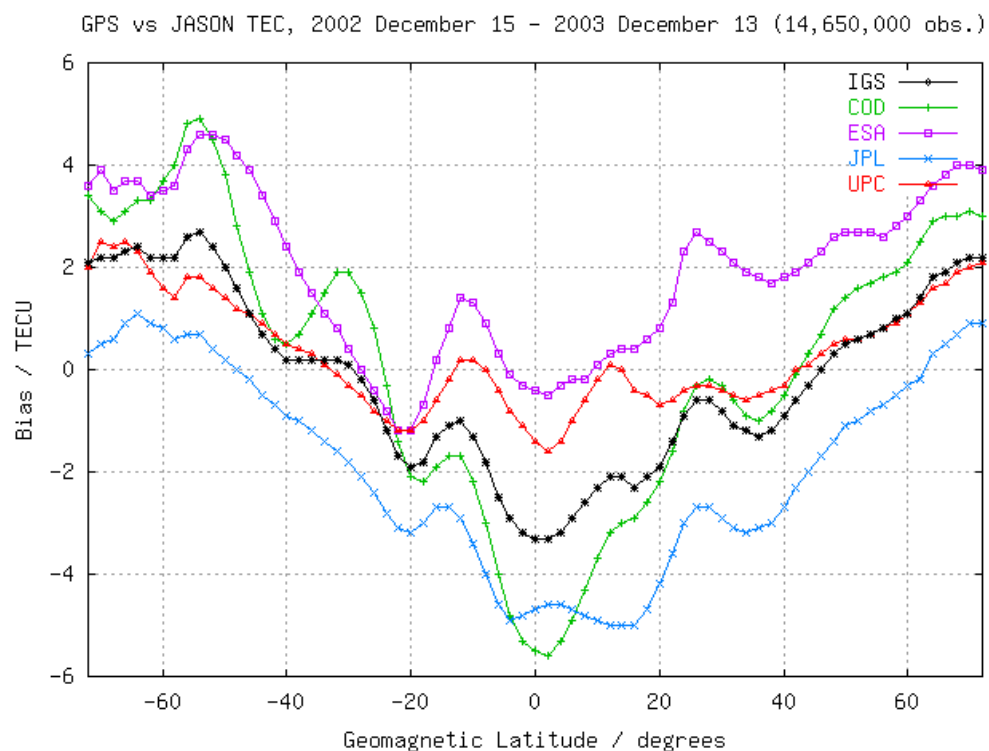
Figure 11: IGS TEC bias regarding to JASON TEC (JASON-IGS), represented as a function of the geomagnetic latitude.
