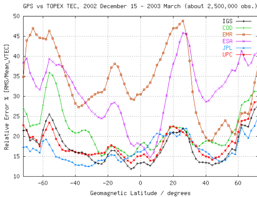
Figure 5: Percentage of “Relative Error” (defined as \text{RMS} \times 100 / \text{Mean Vertical TEC} ) of the GPS TEC maps regarding to TOPEX, as a function of the geomagnetic (2002 Dec. 15th – 2003 March 15th, 2,500,000 TOPEX observations).
