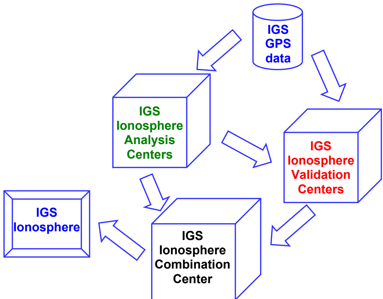
Figure 2: Layout showing the main data flow that leads to the generation of the final IGS Ionospheric product. IGS Final Ionosphere ionex files at ftp://cddisa.gsfc.nasa.gov/gps/products/ionex/ . More details of the IGS final product, including download links at http://gagel52.upc.es/~ionex3/igs_iono/igs_iono.html .
