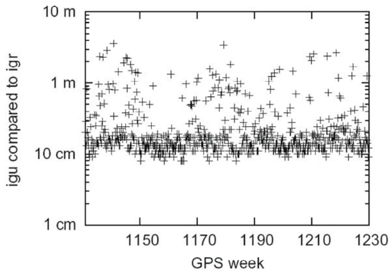
Figure 1: Daily RMS differences – over satellites and the day – between Ultra rapid and rapid orbits. Unless the outliers are flagged with appropriate codes in the sp3c file, points with large differences are problematic and would benefit from integrity monitoring.
